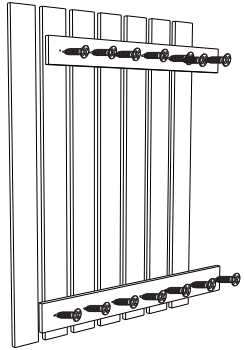
VİDA 3,5X30 MM
